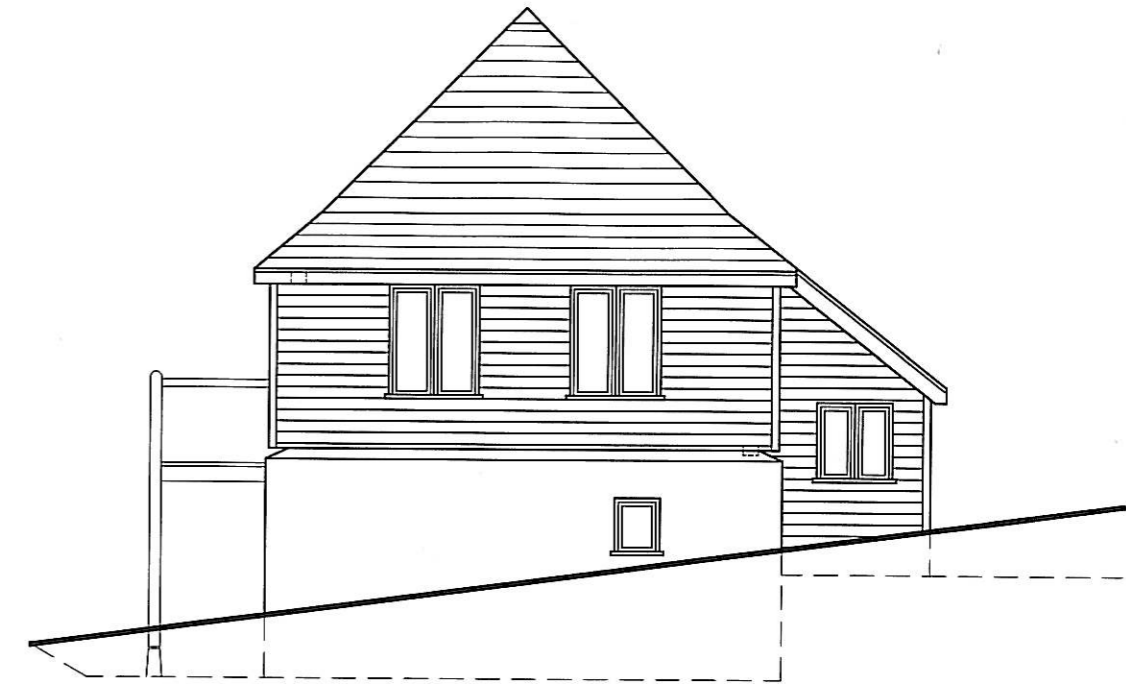
SIDE ELEVATION 1:100
