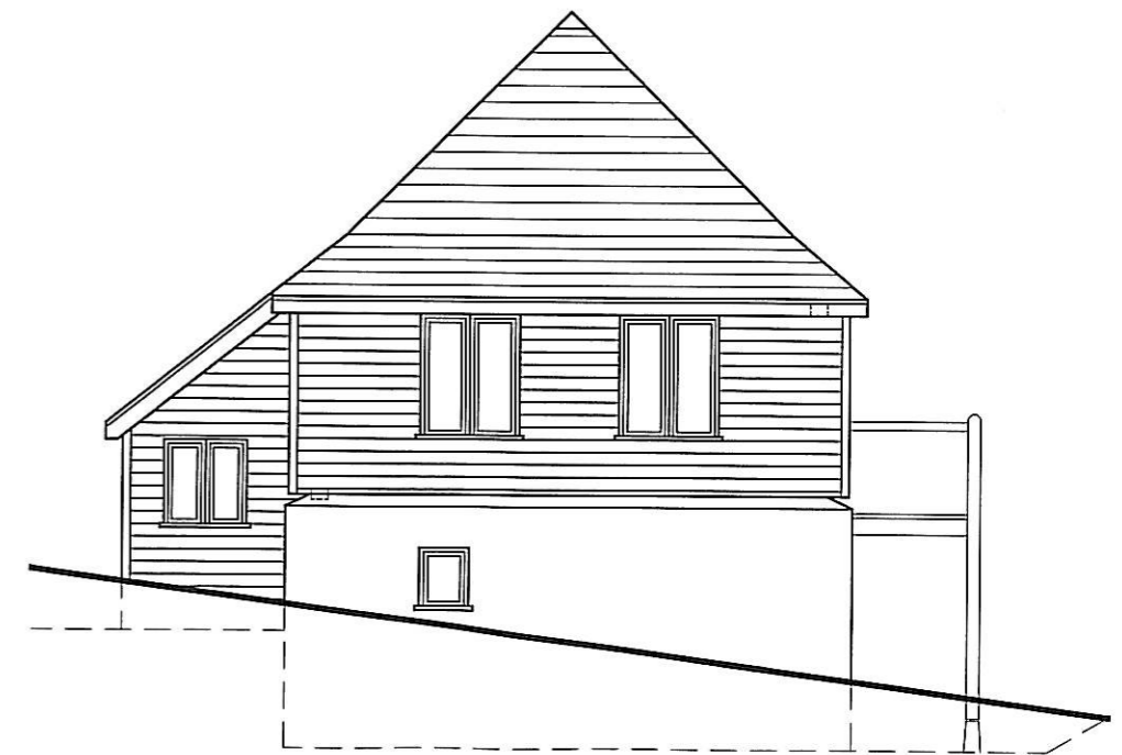
SIDE ELEVATION 1:100
