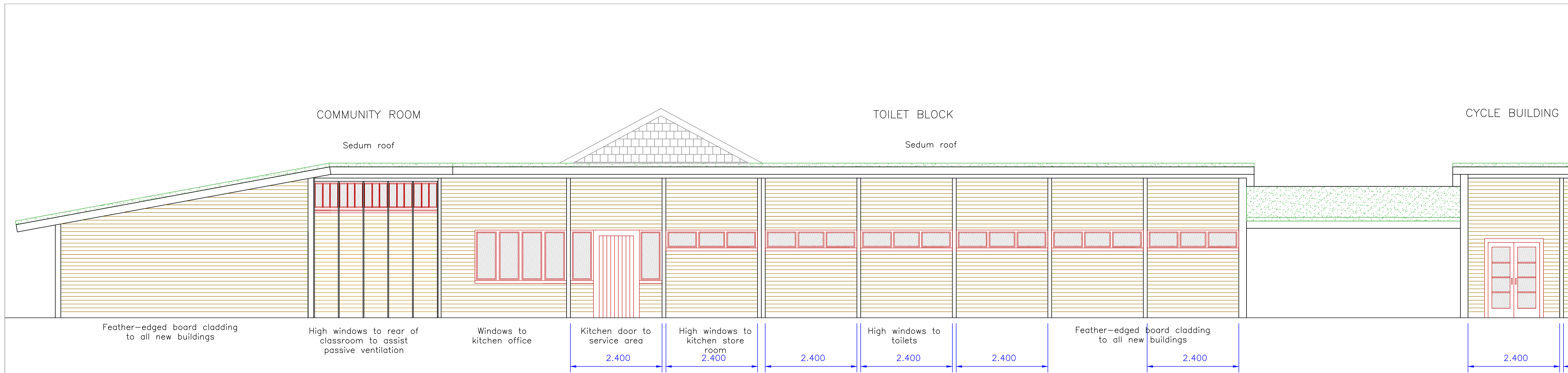
EAST ELEVATION
