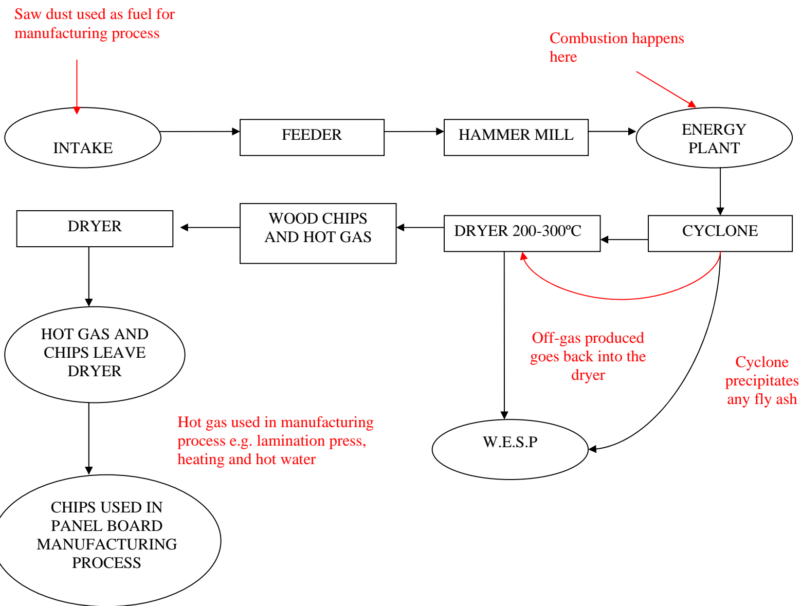
Fig 9.1. Example of the boiler process at Egger UK
