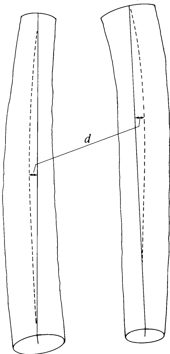
Figure 1 Straightness
