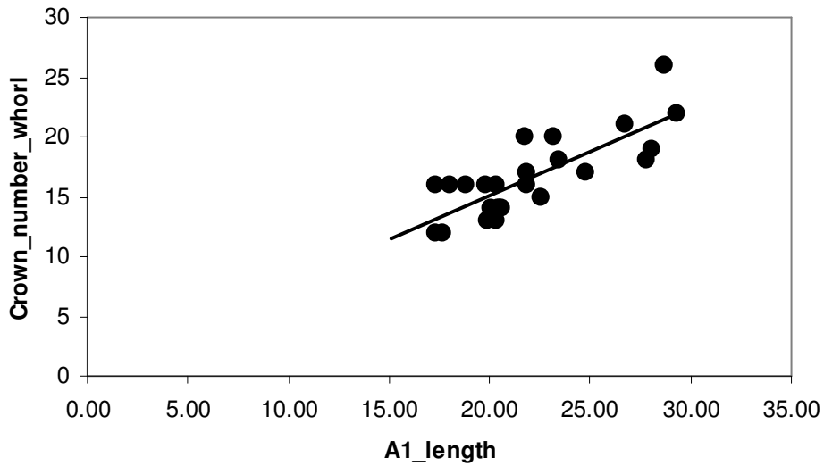
Figure 4. Number of whorl ( nWhorl ) versus the tree height ( IA1 ) (Equation 3). y = 0.74 x + 0.39 , r^2 = 0.63 , n = 27 .
