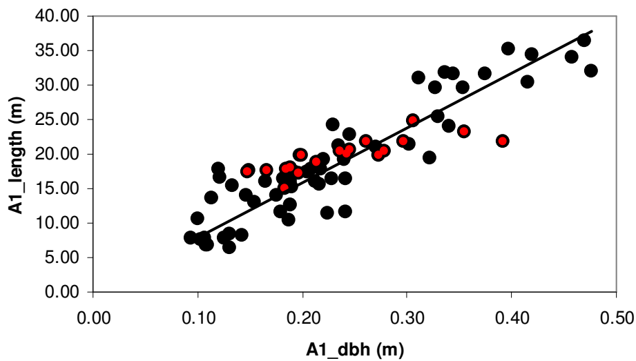
Figure 2. Tree height ( lA1 ) versus tree dbh (Equation 1). Red points are data recorded in this study and black ones from Achim and Gardiner (2005). y = 79.6 x , r^2 = 0.78 .
