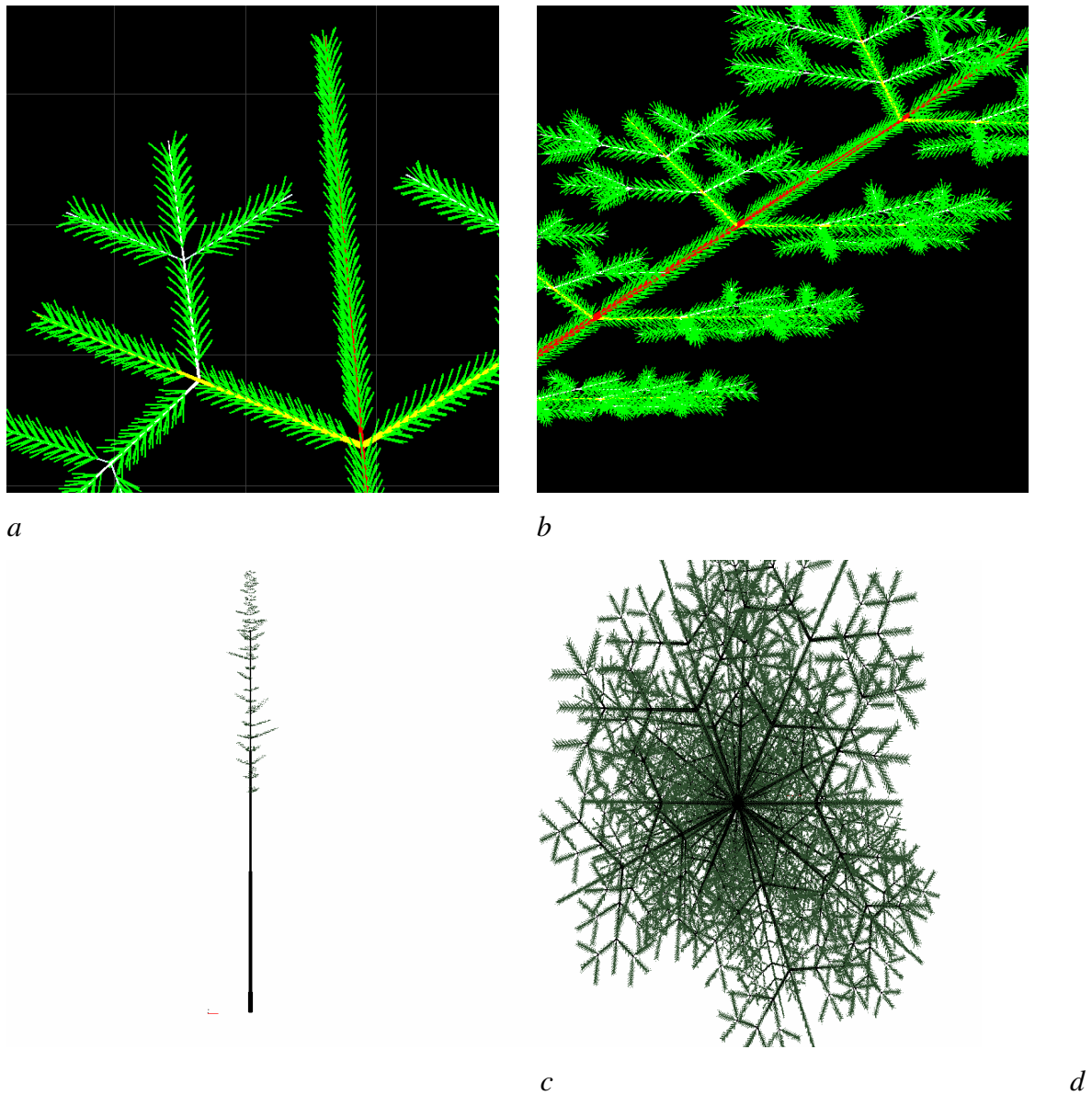
Figure 8. Examples of virtual images, computer-generated from the 3-D SITKA model outputs by the Pov-Ray™ software for a 30-m height Sitka spruce tree. Bottom branch (a and b), south to the north (c) and top-down (d) views.
