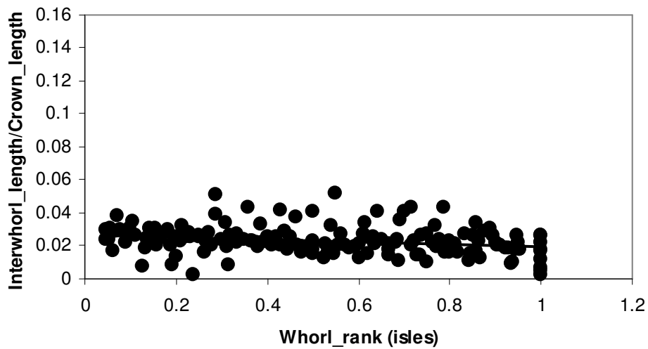
Figure 5. Interwhorl length versus the relative whorl rank on A1 for the forest sites Castlemilk ( y = -0.068 x + 0.11 , r^2 = 0.42 ), Ryes ( y = -0.021 x + 0.07 , r^2 = 0.11 ), and Isles ( y = -0.007 x + 0.03 , r^2 = 0.06 ) (Equation 4).
