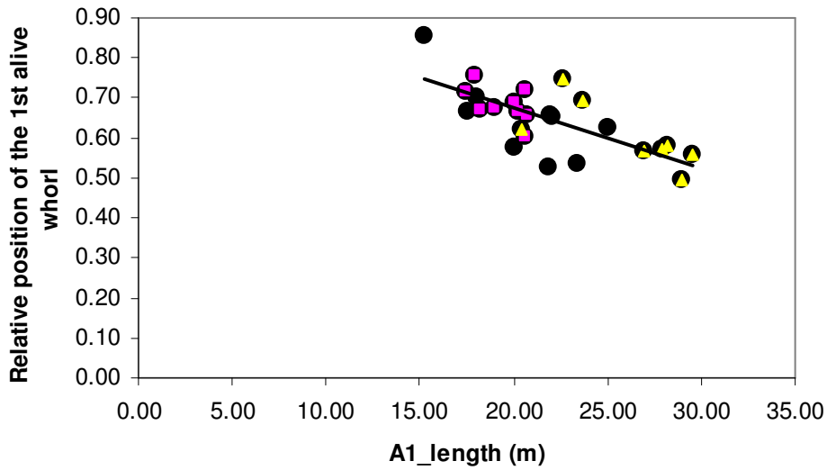
Figure 3. Relative position of the first live whorl on A1 versus its height (Equation 2). In black: Ryes, yellow: Isles and purple: Castlemilk. y = -0.015 x + 0.98 , r^2 = 0.52 , n = 27 .
