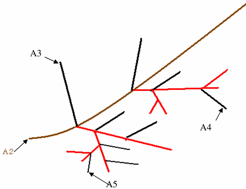
Figure 1. Multi-scale codification of a Sitka branch.
