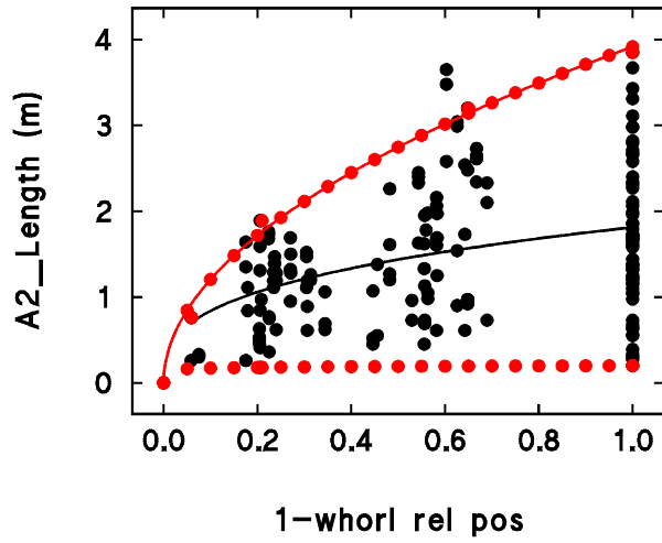
Figure 6. Branch length ( lA2 ) versus the relative position of the whorl within the tree crown (Equation 6).
