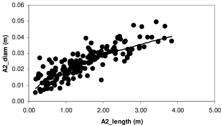
Figure 7. Branches diameter ( dA2 ) versus lA2 (Equation 7). y = 0.02 x^{0.53} , r^2 = 0.64 ,
